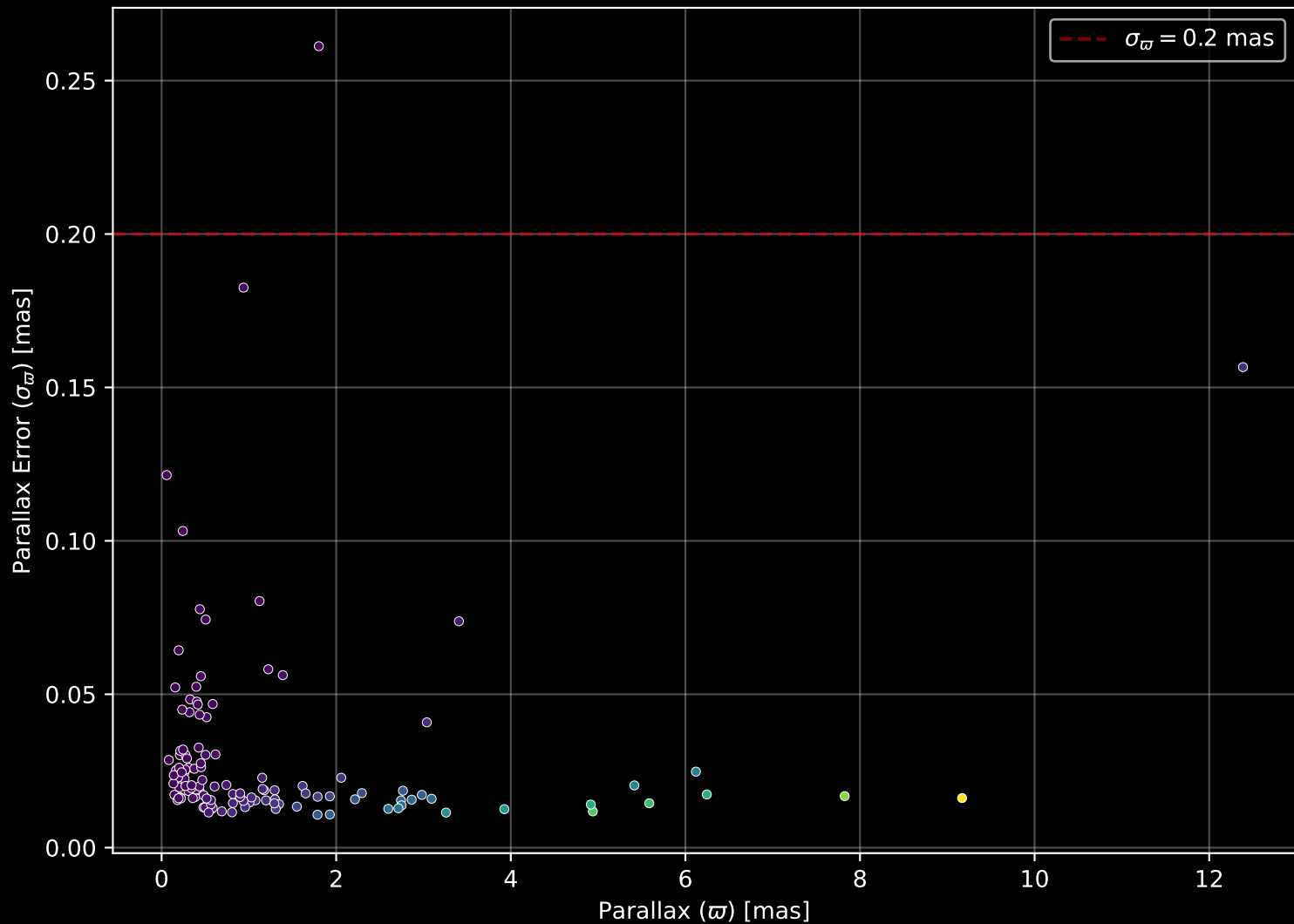
APOGEE DR17 Field: [W5a] Parallax Quality (n= 123)
