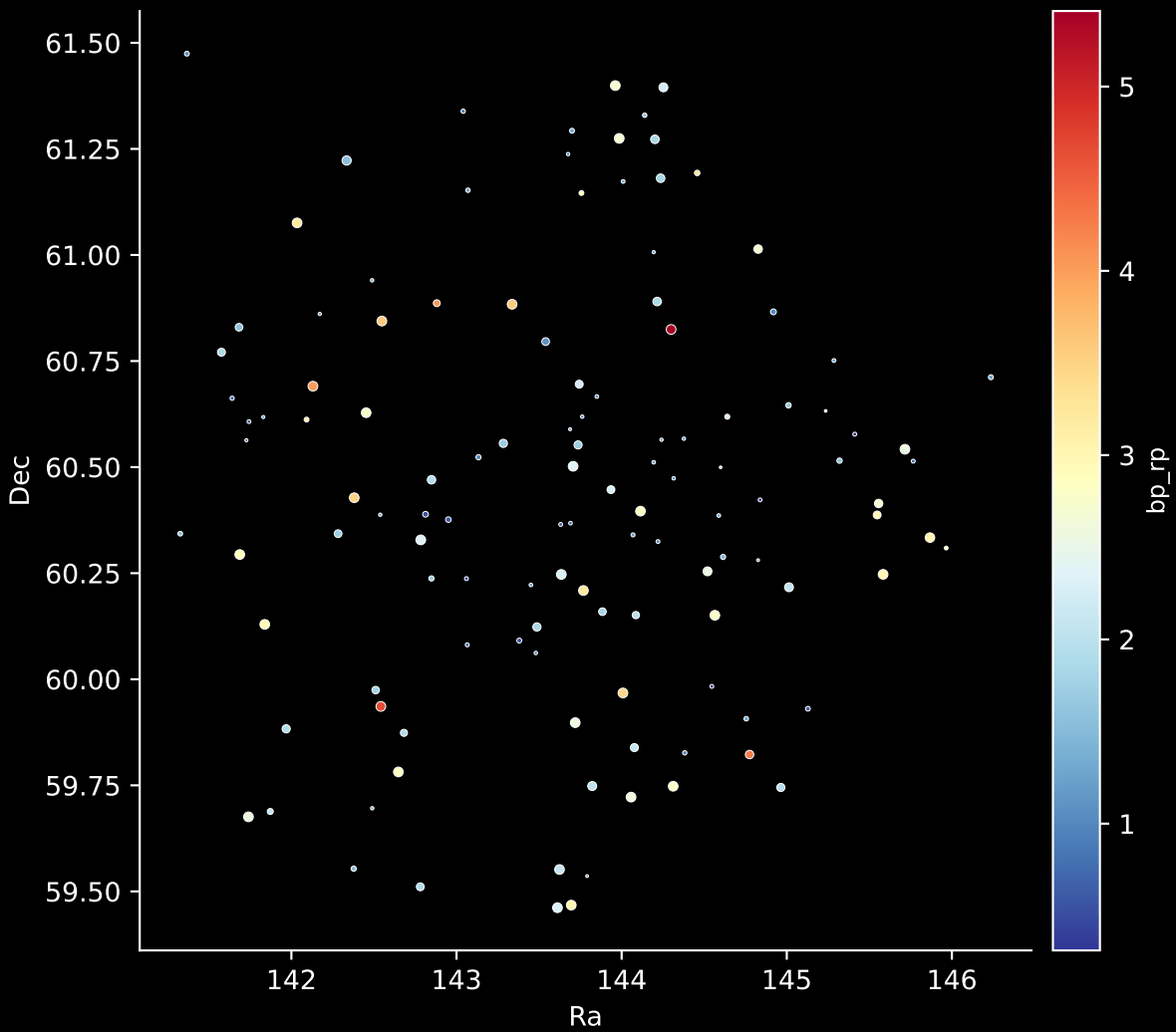
APOGEE DR17 Field: [W5a] Stars: 123
