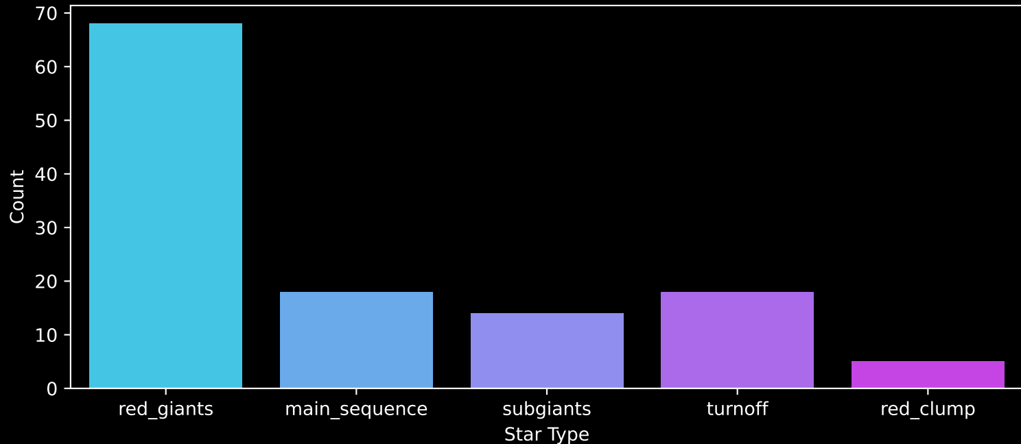
APOGEE DR17 Field: [W5a] Count plot of Star Type
