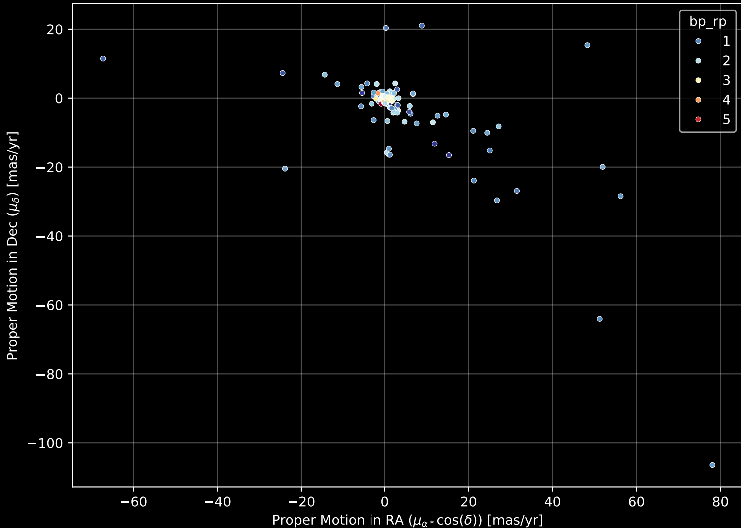
APOGEE DR17 Field: [W5a] Proper Motion Diagram (n= 123)
