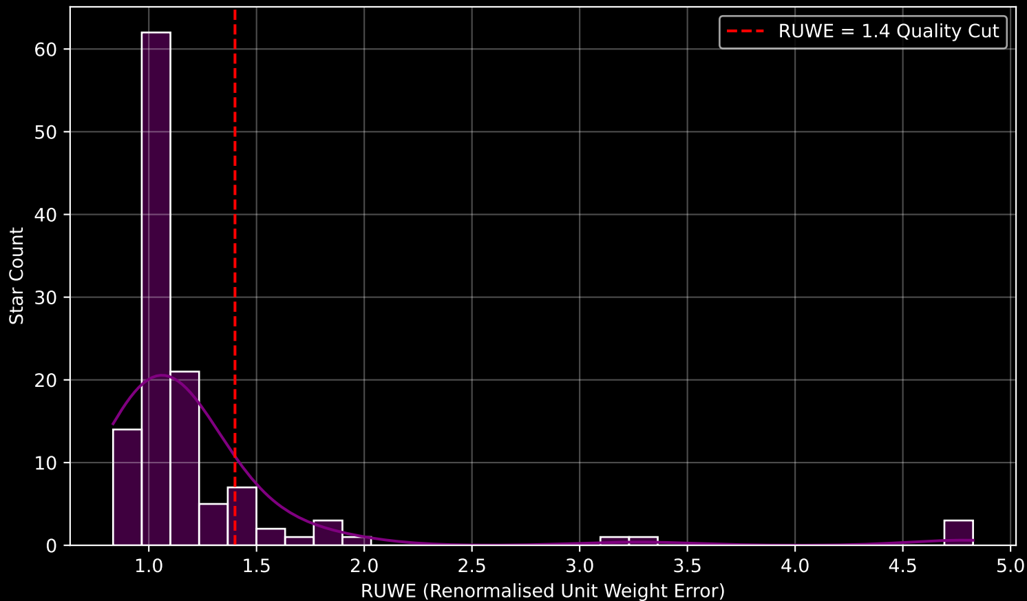
GAPOGEE DR17 Field [W5a] RUWE Distribution (n= 121)
