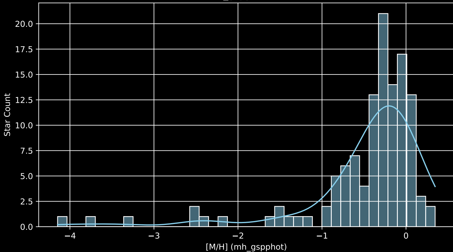
APOGEE DR17 Field: [W5a [M/H] (mh_gspphot) (n= 120)
