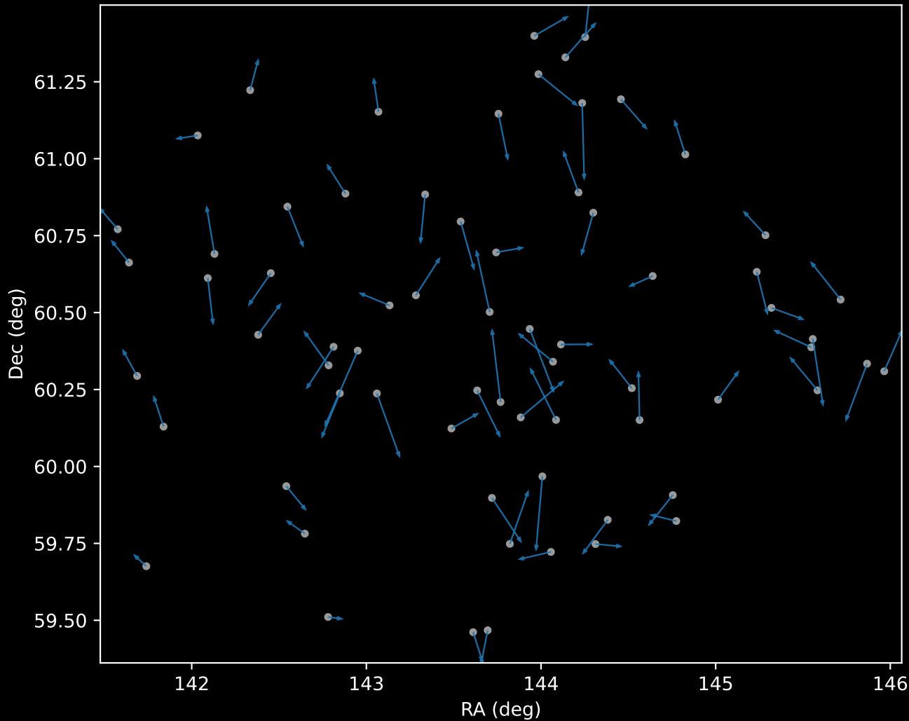
APOGEE DR17 Cluster 0 Proper Motion Vectors (n=69)
